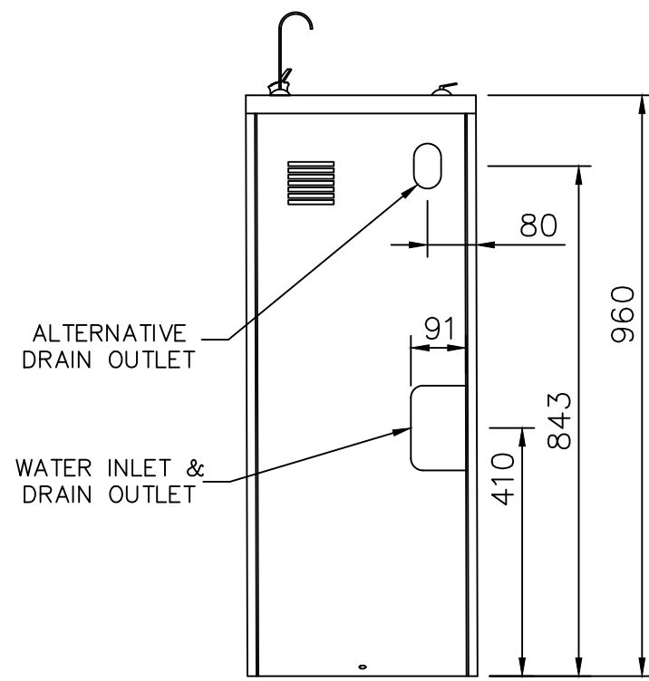
BACK VIEW
